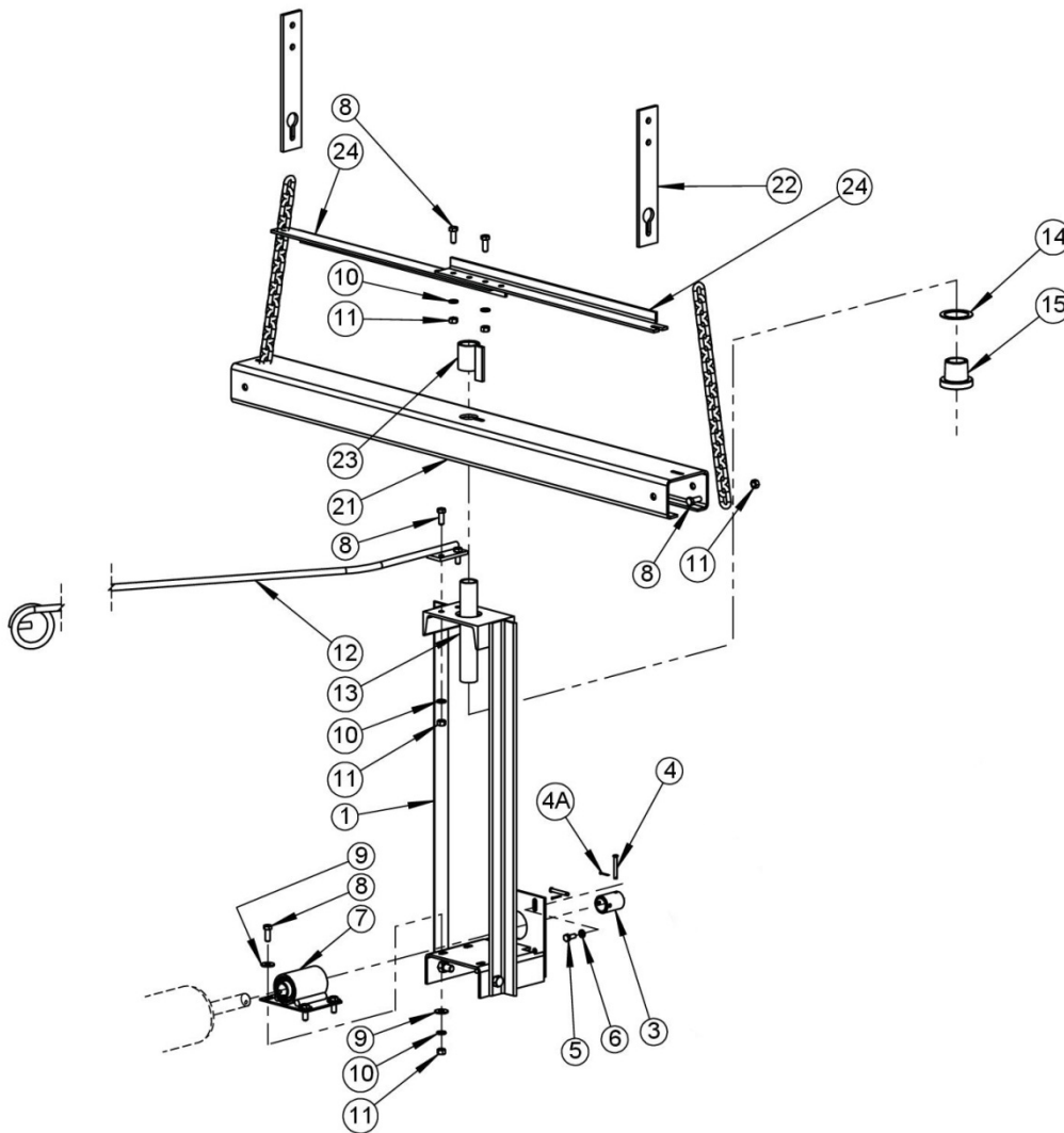
120A00-14-CDK050– Rotating contact for stirring system, 16 pol, 2 + 3 augers.
