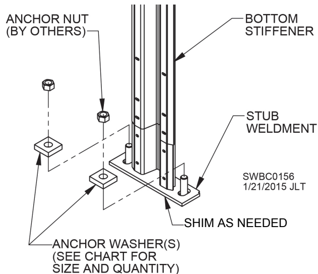
Double-Anchor Boot 72' Dia. and larger (2 Stiffeners/Sidewall Sheet)
