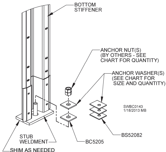
Single-Anchor Boot 69' Dia. and smaller (2 Stiffeners/Sidewall Sheet) 72' Dia. and larger (3 Stiffeners/Sidewall Sheet)
